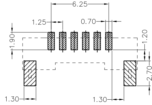
PCB LAYOUT(Tolerance:±0.05)
