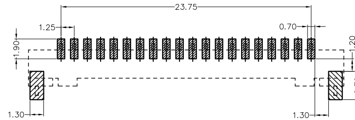
PCB LAYOUT(Tolerance:±0.05)
