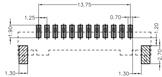
PCB LAYOUT(Tolerance:±0.05)
